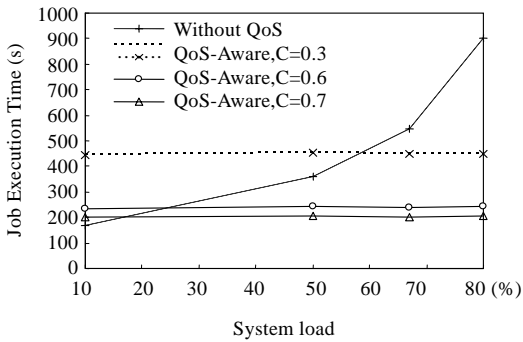
Fig.3 Service execution time at different system load in AREM application
